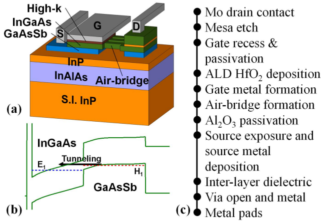
Fig. 1. (a) 3-D schematic view, (b) corresponding simulated ON state band diagram with first subbands of InGaAs and GaAsSb, and (c) process flow of the type-II \text{In}_{0.53}\text{Ga}_{0.47}\text{As}/\text{GaAs}_{0.5}\text{Sb}_{0.5} vertical TFET.
